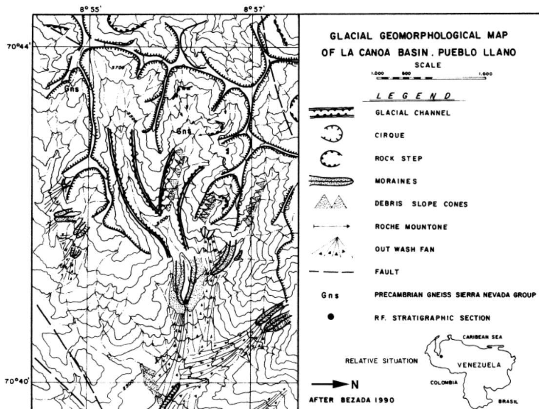
Figure III-4. Example of geomorphological features in the central MA. Geomorphological map for La Canoa at Pueblo Llano (From Bezada, 1990).
