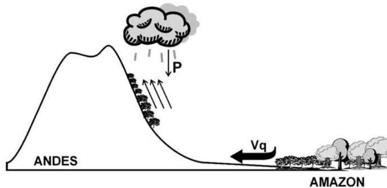
Figure I-4. Schema to show the Amazon basin and rain-forest influence in the central tropical Andes precipitations ( P ) during the May-September. Moisture from the Amazon is transported by the trade winds ( Vq ) (Modified from Poveda et al., 2006).
