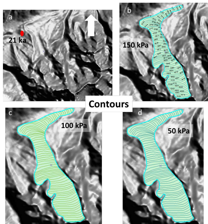
Figure IV-7. Former glacier located in the Mucubají valley at 21 ka and contours drawn. a) The red point shows the sample location and age of the frontal moraine used to draw the former glacier polygon. b), c), d) Former glaciers polygons and contours to each basal shear stress (50, 100 and 150 kPa).
