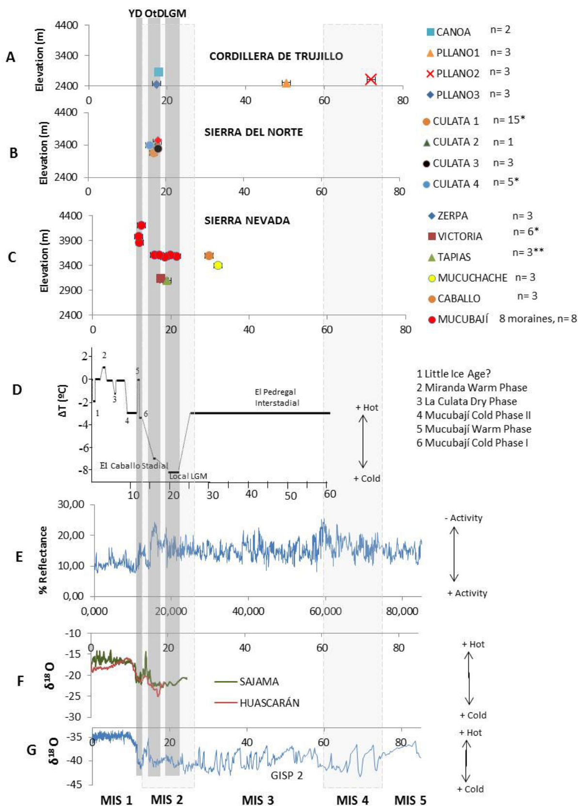
Figure VI-5. Climate forcing driving central Mérida Andes glacier advances. Glacier advances in A) Cordillera de Trujillo, B) Sierra del Norte and C) Sierra Nevada-Sierra de Santo Domingo. D) Temperatures variations in the central Mérida Andes deduced
