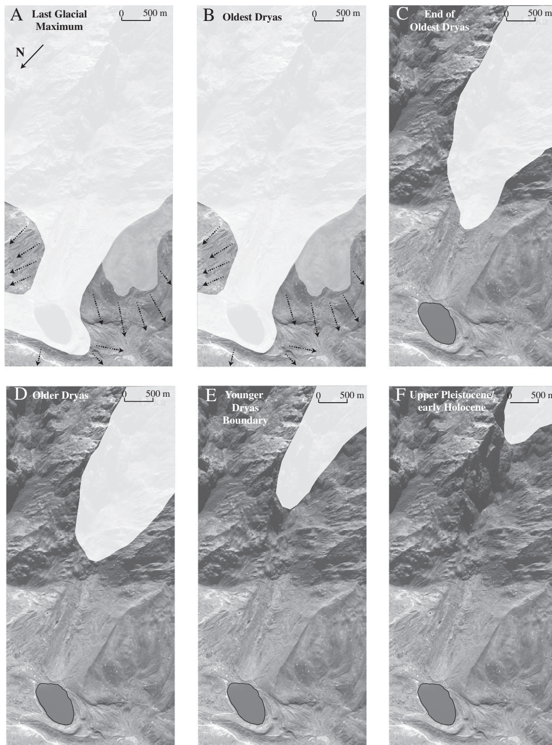
Figure 5. Timeline of the deglaciation in the Mucubají valley. The white cover indicate the glacier extent deduced from the present study, the gray cover indicate the presumed glacier location in the Mesa del Caballo deduced from field work and dating correlations, dashed arrows are the paraglacial outwash sediments.
