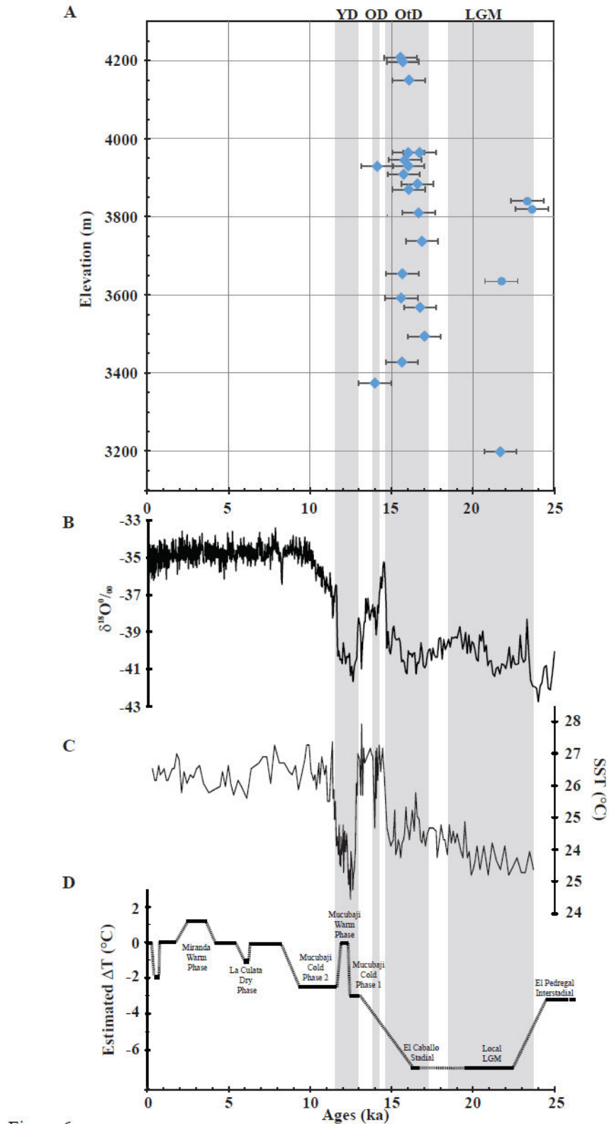
Figure 6. A) Altitudinal relation of the Gavidia glacier chronologies versus global (B), regional (C) and local (D) paleoclimatic proxy records. Dots are samples collected on
